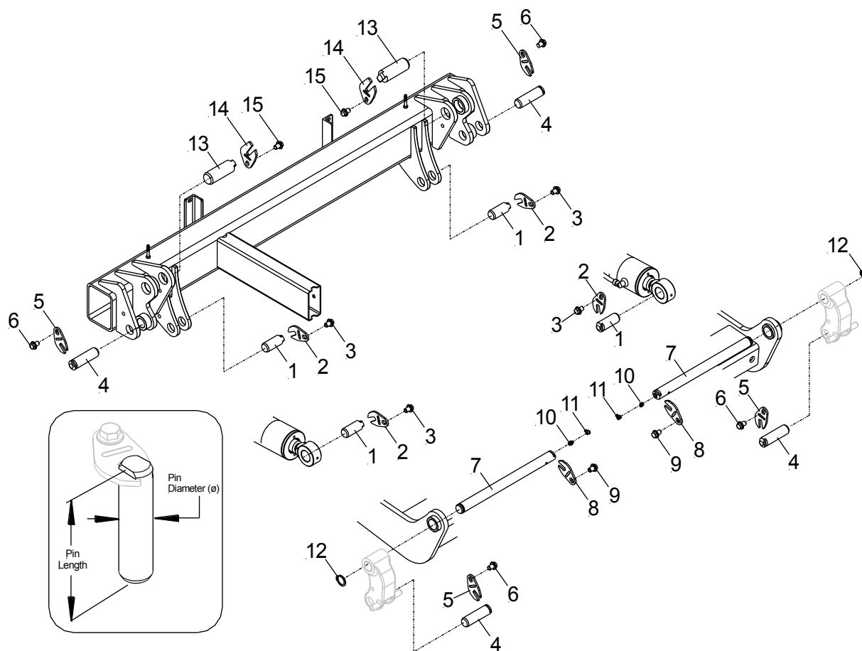
3.2 – DUAL CYLINDER FRAME PINS
