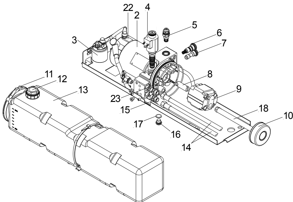
12.2 – PUMP AND MOTOR – ILK 22/33/44/55/66
