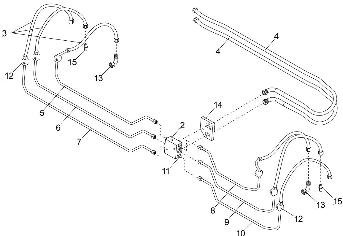
11.3 – HYDRAULIC PIPES – ILK 33,44,55,66
